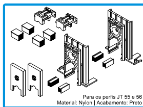
212133 CONJ. TOPOS CENTRAL JT-SLIM
