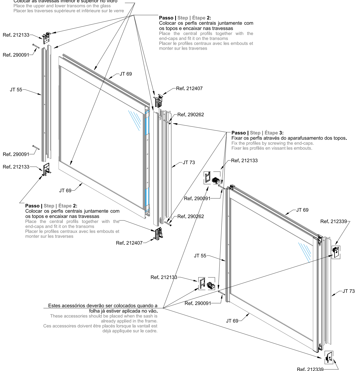
212133 CONJ. TOPOS CENTRAL JT-SLIM
