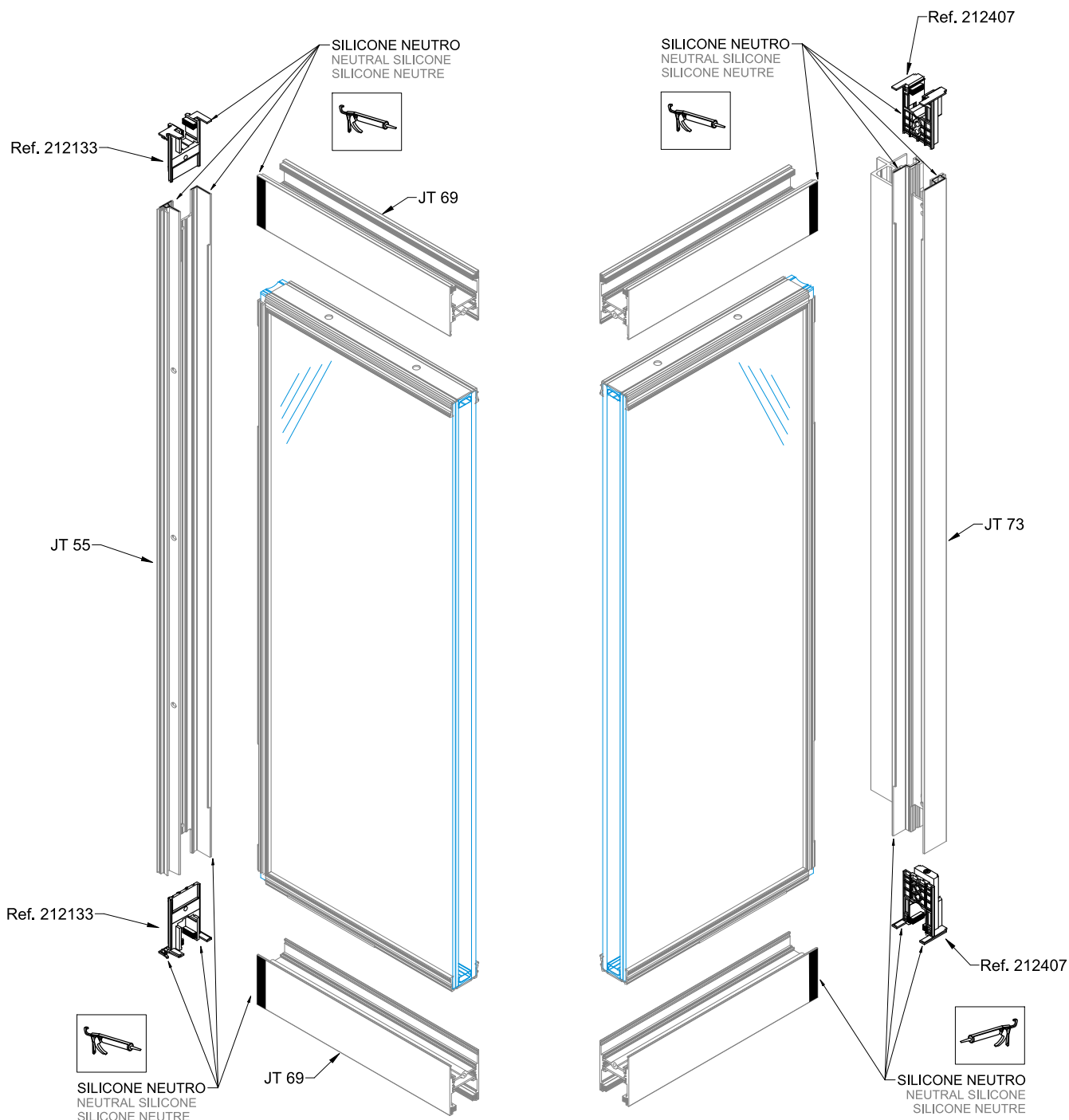
212133 CONJ. TOPOS CENTRAL JT-SLIM
