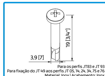
290472 PARAF. AT/PF CQ Ø3.9x19MM A2
