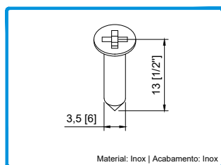
290050 PARAF. DIN7982 PH 3,5x13 INOX A2
