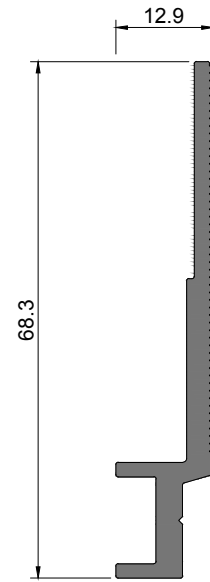
SO 89 Bite Bead | Parclose
