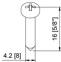
290088 PARAF. DIN7981 PH 4,2x16 INOX A2
