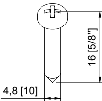
290064 PARAF. DIN7981 PH 4,8x16 INOX A2
