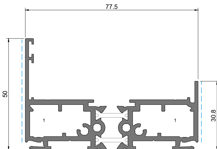
SO 55 Ombreira/padieira 1-rail 1-rail Door jamb/lintel | Jambage/linteau 1-rail
