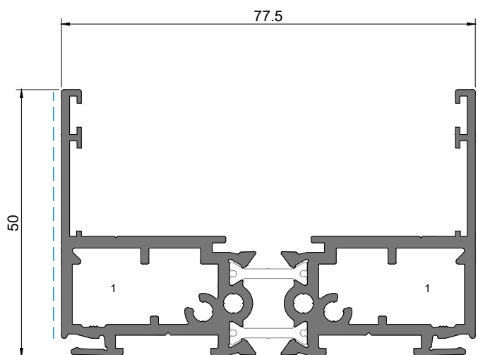
SO 44 Ombreira/padieira 1-rail 1-rail Door jamb/lintel | Jambage/linteau 1-rail
